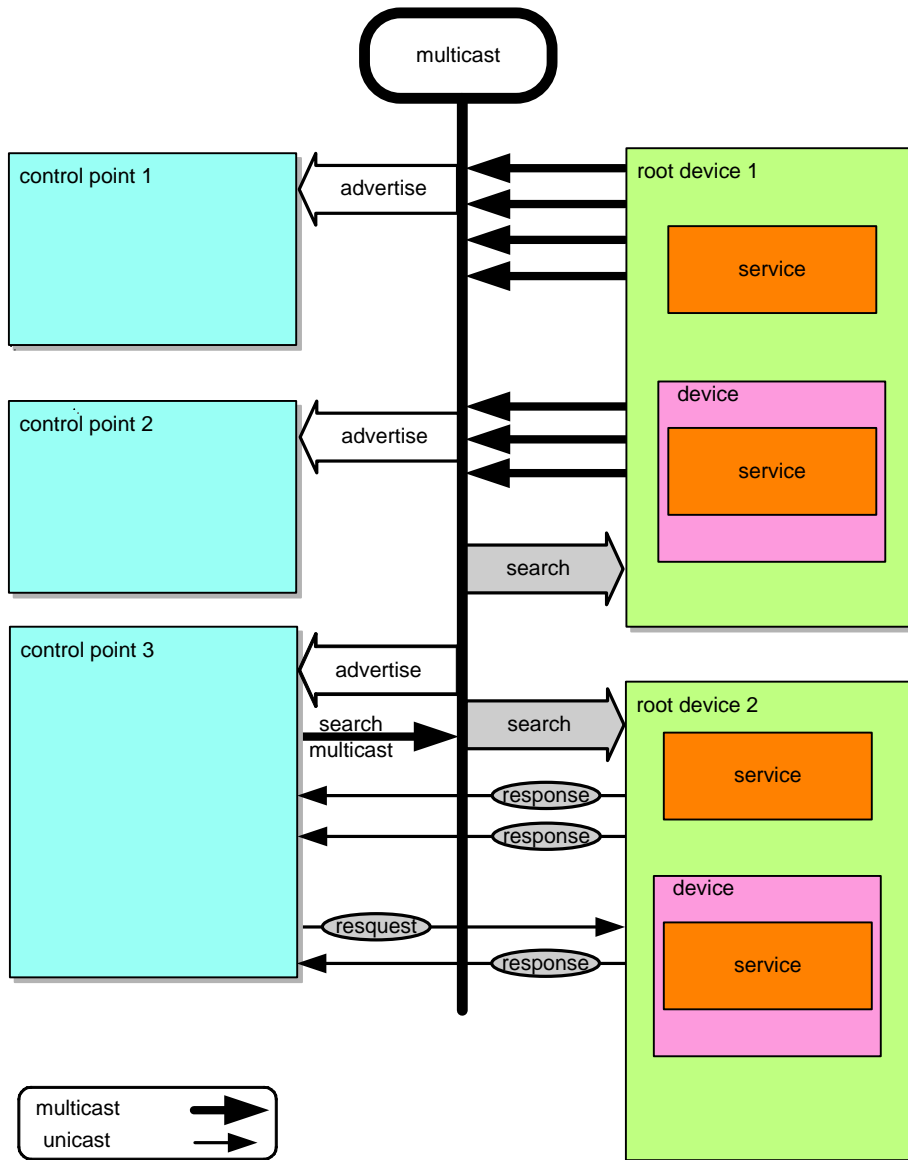
Figure 1-1: — Discovery architecture
