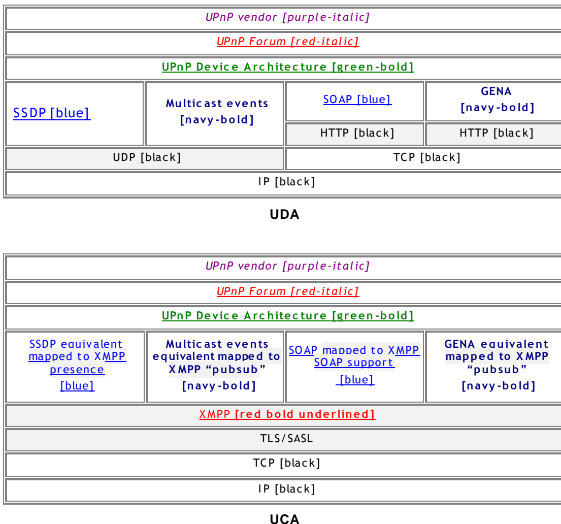
Figure C-1: — Protocol stacks UDA versus UCA 8
