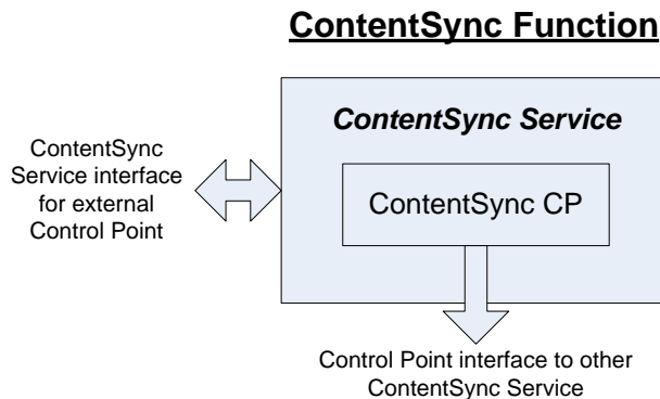
Figure 4 ContentSync Function
