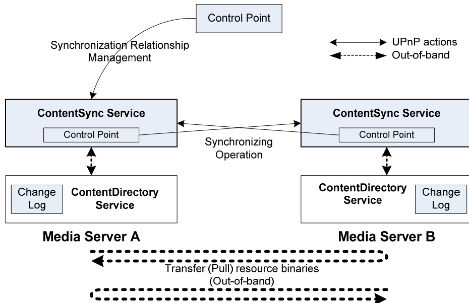
Figure 1 Content Synchronization Model
