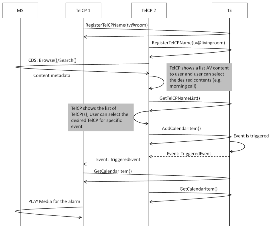
Figure B.3 — Multiple TelCP handling for Alarm use case
